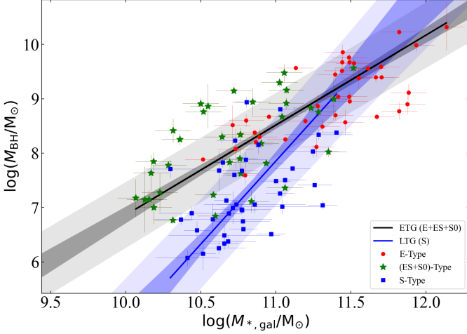
Fig. 2. Black hole mass versus total galaxy stellar mass. This diagram has two distinct relations defined by (all) ETGs and LTGs (see Equations 5 and 6).
