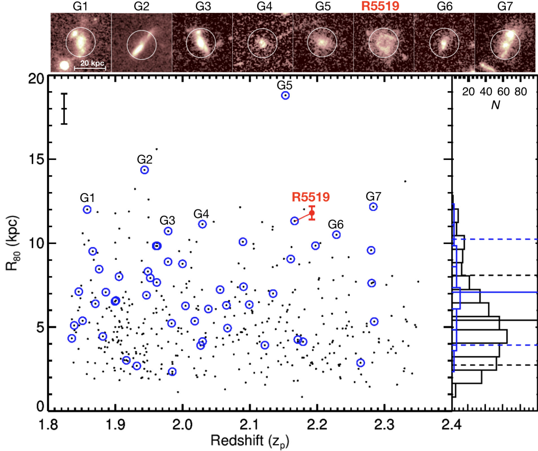
Figure 3 – Comparing the size of R5519 with the size distribution of late-type galaxies at z \approx 2 . The z_p and R_{80} values are from the 3D-HST survey and its mass-size catalogue in the COSMOS field (Methods). The typical error bar for R_{80} , defined as an average error propagated through the 1\sigma model error of the effective radius in 3D-HST, is shown in the top left corner. The black dots show all galaxies with \log(M_*/M_\odot) \geq 9.5 . The blue circles highlight the most massive objects, defined as \log(M_*/M_\odot) \geq 10.6 . The histograms (right) show the size distribution for all (black) and the most massive (blue) galaxies. The horizontal solid and dashed lines mark the mean and the 1\sigma scatter of the size distributions. Including R5519, there are eight objects (labelled G1-G8) that have unusually large sizes (defined as 1\sigma above the mean size of the most massive galaxies). The F160W band morphologies for these eight objects are shown as postage-stamp images at the top. The red filled circle shows z_s and our non-parametric measurement of R_{80} for R5519. We note that the inferred R_{80} for the 3D-HST sample is based on an empirical relation for a large sample of galaxies; individual galaxies may deviate from this relation due to scatter (Methods).
