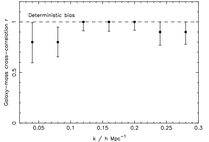
Figure 9. The galaxy-mass cross-correlation parameter r as a function of scale k , measured by fitting Equation 14 to the WiggleZ power spectrum data assuming the growth rate predicted by \Lambda\text{CDM} and marginalizing over linear bias and variable damping factors. The measurements in different redshift slices are combined.
