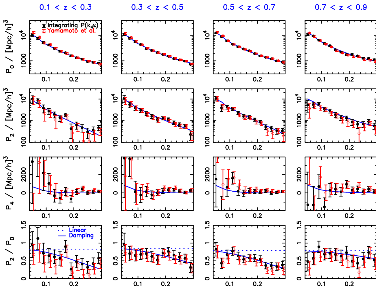
Figure 10. The multipole power spectra P_\ell(k) for \ell = 0, 2, 4 for WiggleZ survey observations in four redshift slices. The monopole ( \ell = 0 ) spectrum primarily contains information about the underlying shape of the isotropic clustering pattern. The quadrupole ( \ell = 2 ) spectrum holds the leading-order signal from the anisotropic modulation in power due to redshift-space effects. The (black) solid circles are generated from the stacked measurements of P_g(k, \mu) across the different survey regions using Equation 17. The (red) open circles, which are offset slightly in the x -direction for clarity, are generated by combining the estimates of P_\ell(k) in each region using the Yamamoto et al. estimator of Equation 19. The model lines correspond to the best-fitting non-linear empirical Lorentzian redshift-space distortion model in each case. The bottom row displays the quadrupole-to-monopole ratio P_2(k)/P_0(k) . Two models are overplotted: the large-scale Kaiser limit predicted in a \Lambda CDM cosmological model with \Omega_m = 0.27 , labelled as “Linear”, and the non-linear redshift-space distortion model, labelled as “Damping”.
