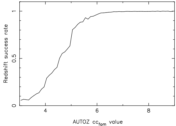
Figure 5. Redshift success rate of 2dFLenS observations, defined by the fraction of spectra with redshift quality flag \geq 3 , as a function of the cross-correlation parameter cc_{tom} determined by the AUTOZ code.
