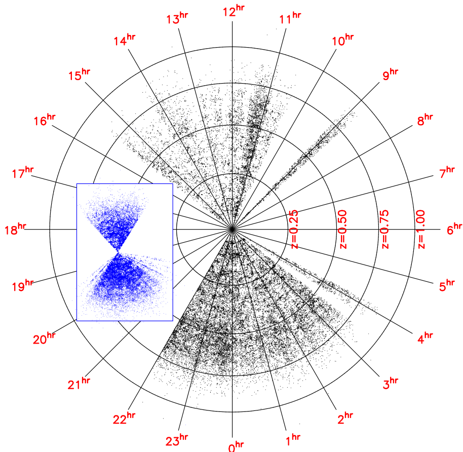
Figure 7. Illustration of the distribution of large-scale structure in 2dFLENs, generated by projecting the galaxy positions by right ascension and co-moving distance, indicated by the black points. The blue points in the inset display on the same scale the earlier 2dFGRS dataset (Colless et al. 2001) obtained by the AAT.
