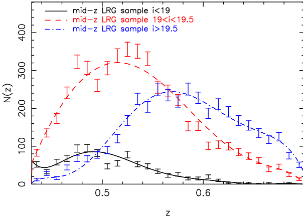
Figure 12. The redshift distribution of the mid-z LRG sample in i -band magnitude bands, together with Chebyshev polynomial fits.
