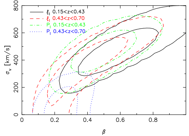
Figure 21. Confidence regions of fits for \beta and \sigma_v , marginalizing over b . Results are shown for fits to both correlation function and power spectrum multipoles, for two redshift ranges 0.15 < z < 0.43 and 0.43 < z < 0.70 . 68% and 95% confidence regions are shown in all cases.
