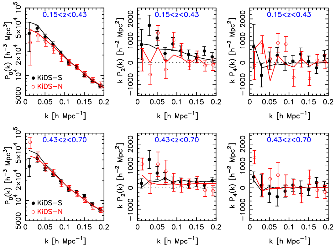
Figure 18. The multipole power spectra ( P_0, P_2, P_4 ), from left-to-right, for 2dFLenS LRGs in the KiDS-S (black solid circles) and KiDS-N (red open circles) regions. Results are shown for two redshift ranges 0.15 < z < 0.43 (top row) and 0.43 < z < 0.7 (bottom row). The solid lines indicate the best-fitting model convolved in each case with the region window function, which produces the ‘choppy’ appearance in the model.
