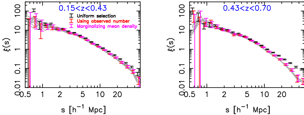
Figure 10. Illustration of our clustering analysis marginalizing over the unknown mean galaxy density in each ATLAS field, for the case of the 2-point correlation function \xi(s) in the KiDS-S region in the two redshift ranges 0.15 < z < 0.43 (left panel) and 0.43 < z < 0.7 (right panel). The black data points are measurements assuming a uniform selection function, neglecting the systematic target density variations, and contain large-scale systematic errors. These may be corrected using the observed number density in each tile as the angular selection, which produces the red data points. The set of grey lines is an ensemble of clustering measurements in which the selection function is statistically sampled from a distribution defined by the observed number and clustering strength. The magenta data points show the mean of this distribution, adding the density systematic error in quadrature to the original error. Measurements for the different cases are slightly shifted along the x -axis for clarity.
