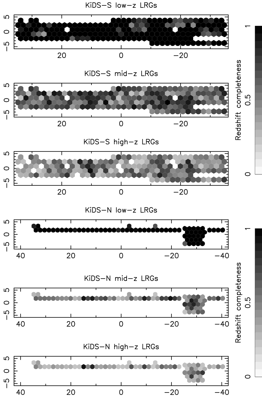
Figure 11. Greyscale map showing the redshift completeness of 2dFLenS observations in the KiDS-S (top 3 rows) and KiDS-N (bottom 3 rows) regions. The x - and y -axes plot separation in degrees from the field centre.
