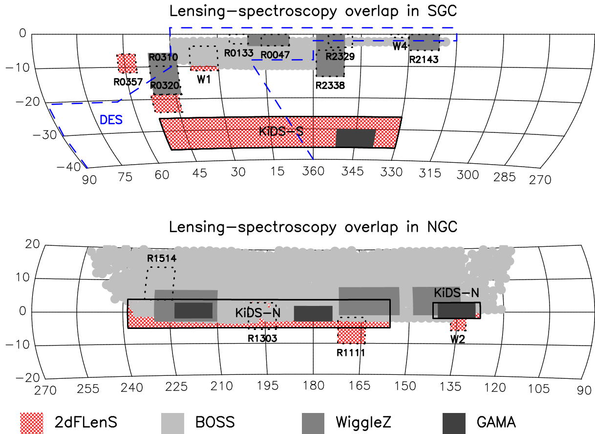
Figure 1. Locations of current spectroscopic and imaging surveys in the Southern Galactic Cap (SGC) and Northern Galactic Cap (NGC). Deep spectroscopic surveys (BOSS, WiggleZ and GAMA) are indicated as grey shaded regions. Deep imaging surveys (CFHTLS, RCS2 and KiDS) are displayed as outlined rectangles, labelled by field names. The approximate DES footprint is located inside the dashed blue line. The originally-planned 2dFLenS spectroscopic coverage is displayed using cross-hatched red shading and spans almost 1000 deg 2 .
