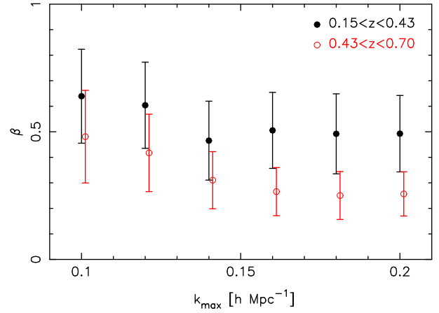
Figure 20. Dependence of the marginalized measurements of \beta on the maximum wavenumber used when fitting the 2dFLenS power spectrum multipole data. Results are shown for the two redshift ranges 0.15 < z < 0.43 (solid black circles) and 0.43 < z < 0.70 (open red circles). Measurements for the different redshifts are slightly shifted along the x -axis for clarity.
