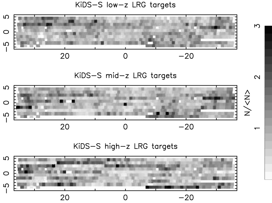
Figure 9. Greyscale map showing the number of LRG targets selected in each ATLAS field in the KiDS-S region, relative to the mean. Significant field-to-field variations are apparent, resulting from photometric zero-point errors. The x - and y -axes plot separation in degrees from the field centre.
