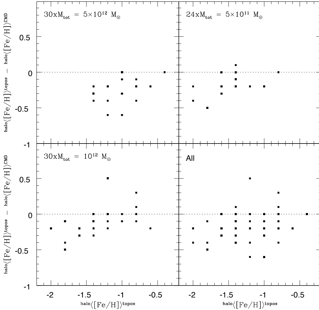
Figure 3.20: The discrepancy in metallicity between \text{halo}\langle[\text{Fe}/\text{H}]\rangle^{\text{topos}} (the “topographical” halo metallicity) and \text{halo}\langle[\text{Fe}/\text{H}]\rangle^{\text{CMD}} (the “topographical” halo metallicity as derived from the halo simulated CMD via metallicity–colour relationship) as a function of the “topographical” halo metallicity.
