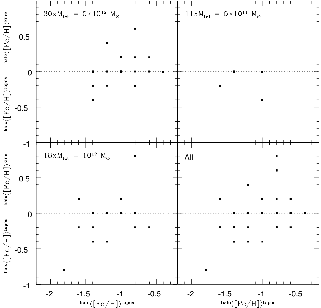
Figure 3.12: The discrepancy between \text{halo}\langle[\text{Fe}/\text{H}]\rangle_{\text{topos}} (the “topographical” halo metallicity) and \text{halo}\langle[\text{Fe}/\text{H}]\rangle_{\text{kine}} (the metallicity of the ensemble of counter-rotating stellar particles within each topographical halo) as a function of the “topographical” halo metallicity.
