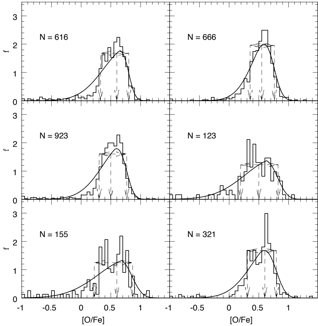
Figure C.8: (continued) Halo stellar particle [O/Fe] distribution for the M_{\text{tot}} = 10^{12} M_{\odot} semi-cosmological simulations in Renda et al. (2005b). The 68% Confidence Level range and the number of stellar particles each distribution refers to are also shown.
