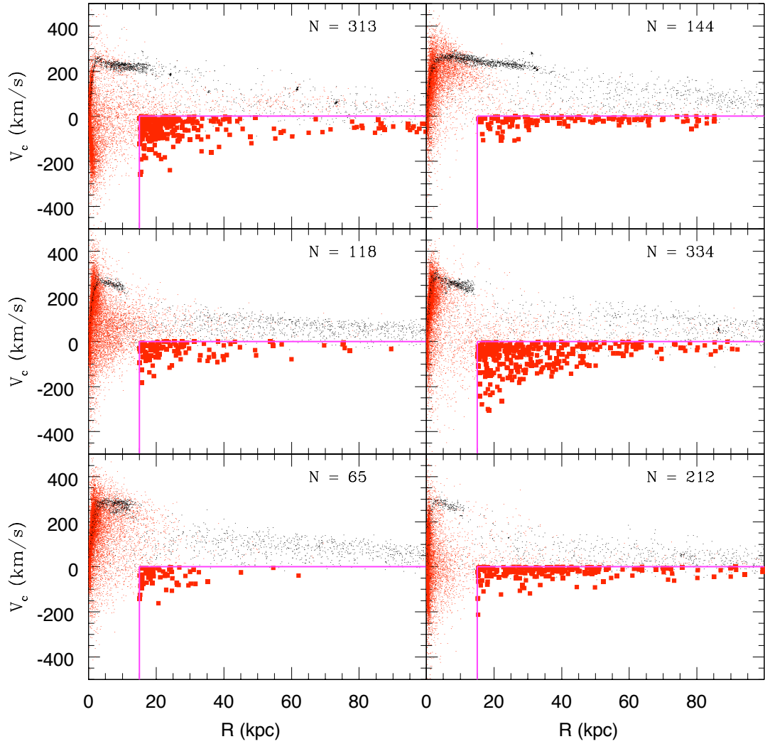
Figure E.6: (continued) Galaxy rotation curves for the M_{\text{tot}} = 10^{12} M_\odot semi-cosmological simulations in Renda et al. (2005b). Black dots for the gaseous particles. Red dots for the stellar particles; red boxes for the ensemble of stellar particles (enclosed within the magenta frame) which are counter-rotating with v_\theta < 0 within each topographical halo at a projected radius R > 15 kpc. The size of such ensemble is also shown in each panel.
