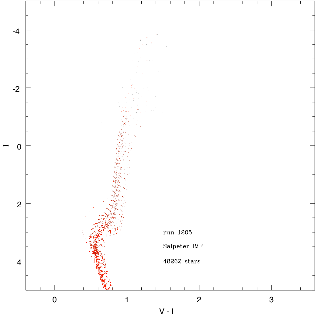
Figure 3.17: Topographical halo simulated CMD for the label “C” semi-cosmological simulation (Figures 3.5 and 3.9) at M_{\text{tot}} 10^{12} M_{\odot} . The observational errors are taken into account (e.g., Secker & Harris 1993) and are randomly drawn for I < -1 from a Normal distribution with \sigma_I = \sigma_V = \exp(I - 0.6) and \sigma_{V-I} = \sqrt{\sigma_I^2 + \sigma_V^2} which implies \sigma_I \approx 0.01 at I = -4.0 and \sigma_I \approx 0.2 at I = -1 whereas at I > -1 \sigma_I = \sigma_V = 0 . Red dots display the simulated CMD without taking observational errors into account. Black dots display the simulated CMD when taking observational errors into account.
