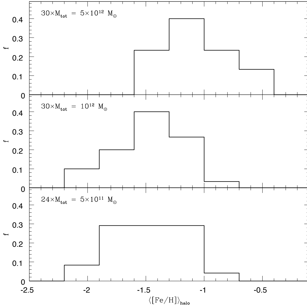
Figure 3.4: Distributions of the z = 0 MDF peaks for the semi-cosmological simulations in Renda et al. (2005b) with M_{\text{tot}} = : 5 \times 10^{11} M_{\odot}; 10^{12} M_{\odot}; 5 \times 10^{12} M_{\odot} .
