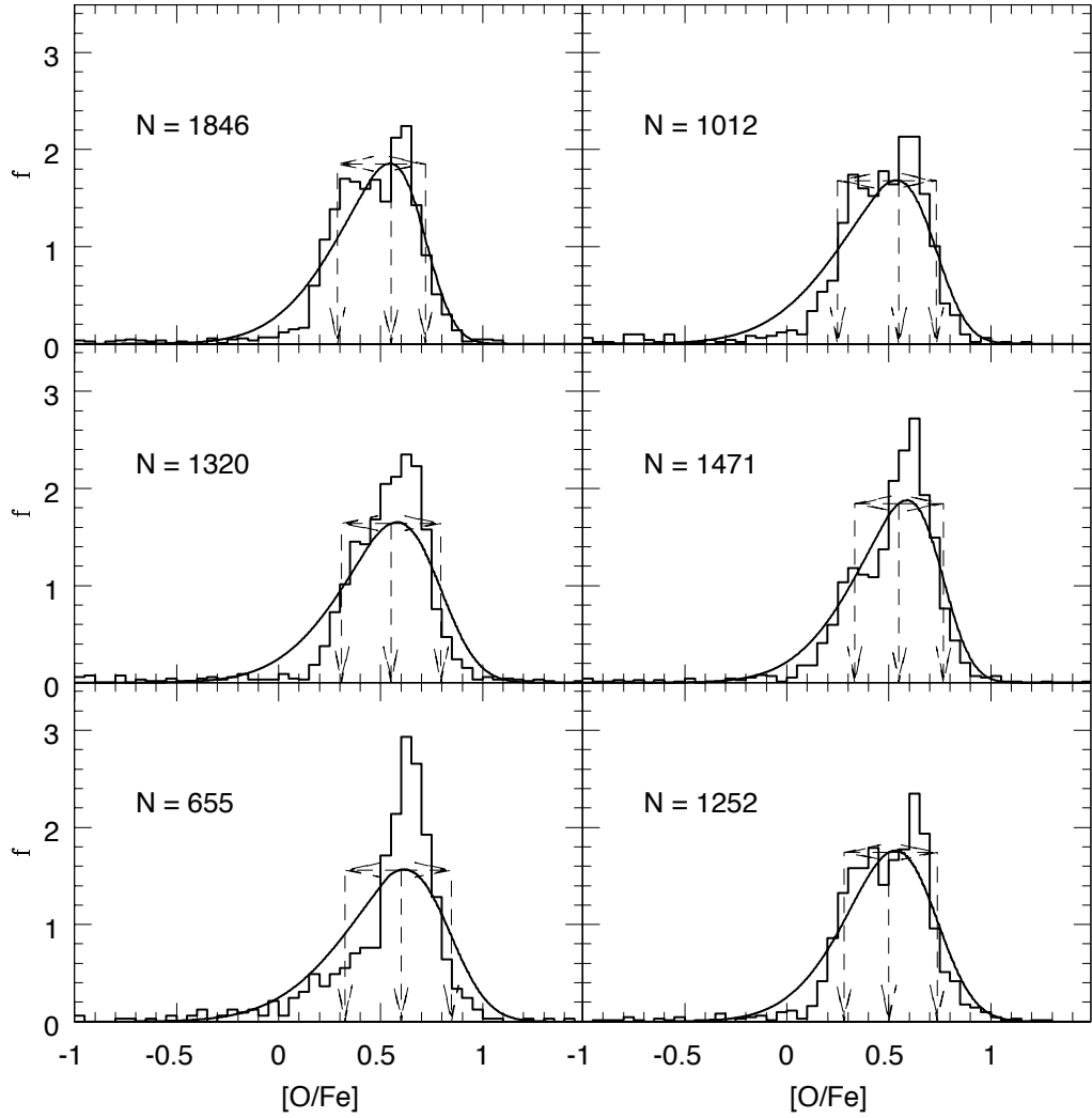
Figure C.12: (continued) Halo stellar particle [O/Fe] distribution for the M_{\text{tot}} = 5 \times 10^{12} M_{\odot} semi-cosmological simulations in Renda et al. (2005b). The 68% Confidence Level range and the number of stellar particles each distribution refers to are also shown.
