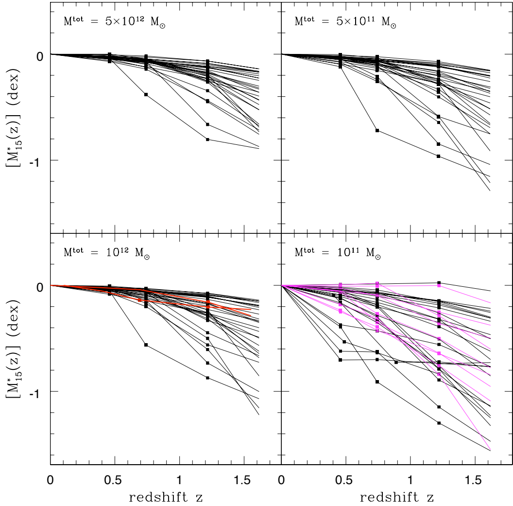
Figure 4.2: The redshift evolution of the stellar mass within the 15 kpc central region, normalised to the z = 0 value for each simulation. The semi-cosmological simulations with collapse redshift z_c = 2 are shown as black lines. Magenta for the collapse redshift z_c = 1.5 runs. The cosmological simulations are shown in red.
