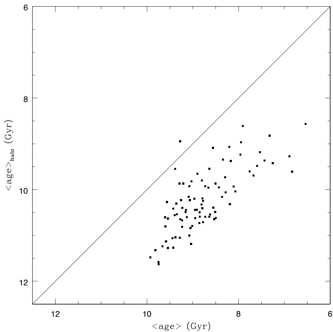
Figure 3.7: The relation between the mean halo age and the mean age for the entire galaxy in our simulations. Both the halo and the galaxy ADFs for each simulation are displayed in Appendix D.
