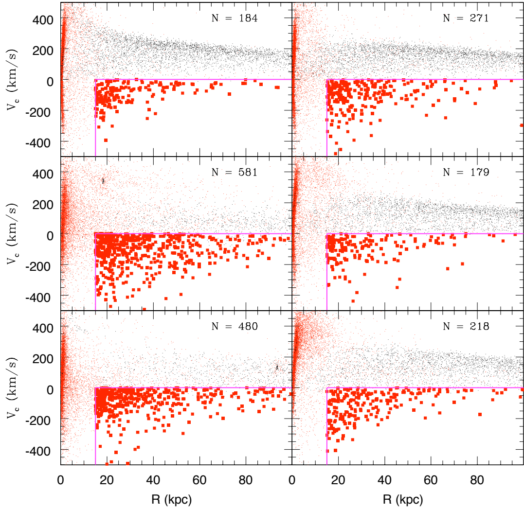
Figure E.14: (continued) Galaxy rotation curves for the M_{\text{tot}} = 5 \times 10^{12} M_\odot semi-cosmological simulations in Renda et al. (2005b). Black dots for the gaseous particles. Red dots for the stellar particles; red boxes for the ensemble of stellar particles (enclosed within the magenta frame) which are counter-rotating with v_\theta < 0 within each topographical halo at a projected radius R > 15 kpc. The size of such ensemble is also shown in each panel.
