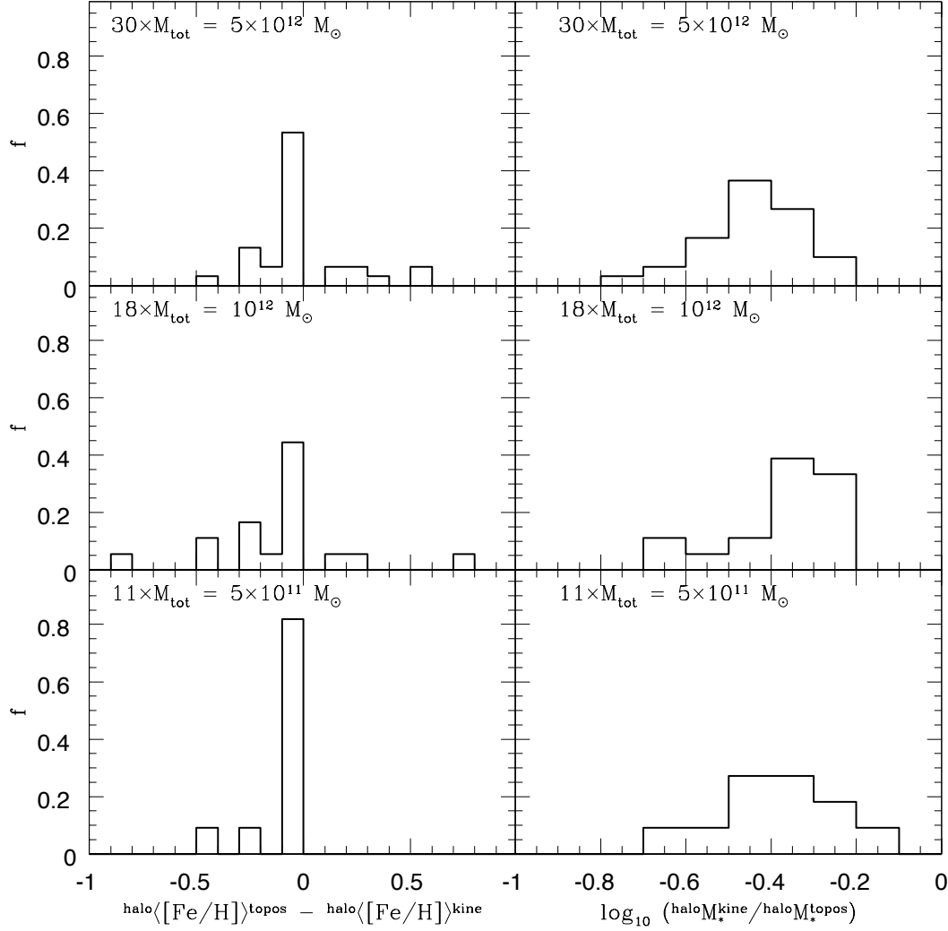
Figure 3.13: Left panels: For each subset, the distribution of the discrepancy between \text{halo}\langle[\text{Fe}/\text{H}]\rangle^{\text{topos}} (the “topographical” halo metallicity) and \text{halo}\langle[\text{Fe}/\text{H}]\rangle^{\text{kine}} (the metallicity of the ensemble of counter-rotating stellar particles within each topographical halo). Right panels: For each subset, the distribution of the “topographical” halo mass fraction the ensemble of its counter-rotating stellar particles amounts to.
