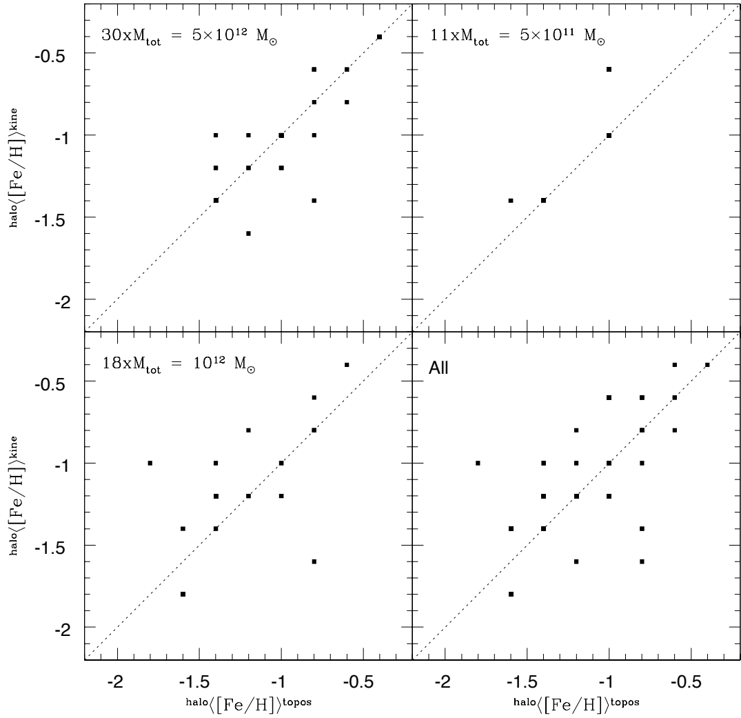
Figure 3.11: The relationship between \text{halo}\langle[\text{Fe}/\text{H}]\rangle^{\text{topos}} (the “topographical” halo metallicity) and \text{halo}\langle[\text{Fe}/\text{H}]\rangle^{\text{kine}} (the metallicity of the ensemble of counter-rotating stellar particles within each topographical halo).
