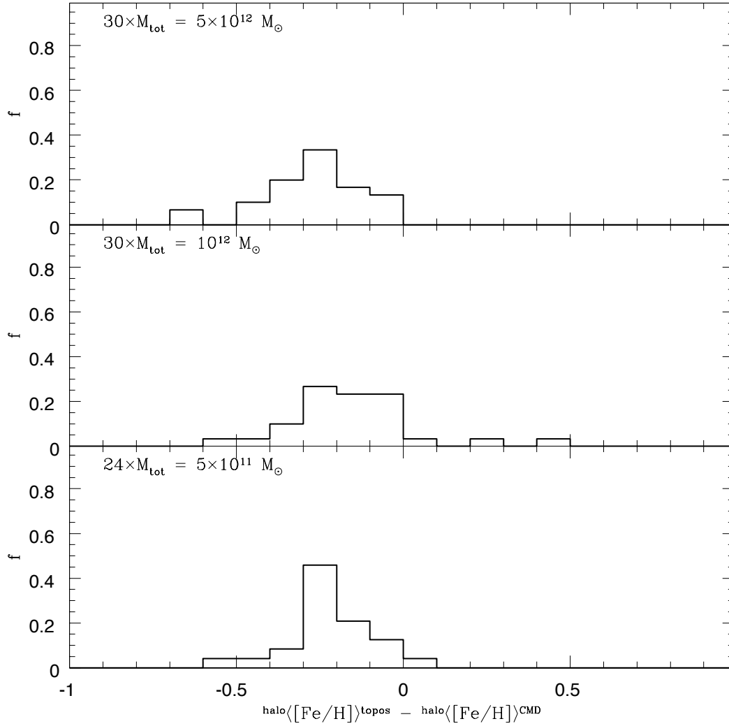
Figure 3.21: For each subset, the distribution of the discrepancy between \text{halo}\langle [Fe/H] \rangle^{\text{topos}} (the “topographical” halo metallicity) and \text{halo}\langle [Fe/H] \rangle^{\text{CMD}} (the “topographical” halo metallicity as derived from the halo simulated CMD via metallicity–colour relationship).
