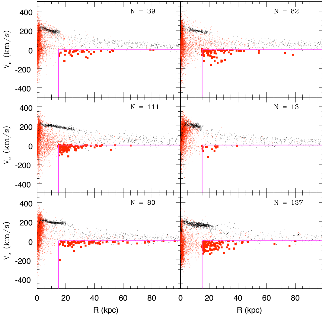
Figure E.1: Galaxy rotation curves for the M_{\text{tot}} = 5 \times 10^{11} M_\odot semi-cosmological simulations in Renda et al. (2005b). Black dots for the gaseous particles. Red dots for the stellar particles; red boxes for the ensemble of stellar particles (enclosed within the magenta frame) which are counter-rotating with v_\theta < 0 within each topographical halo at a projected radius R > 15 kpc. The size of such ensemble is also shown in each panel.
