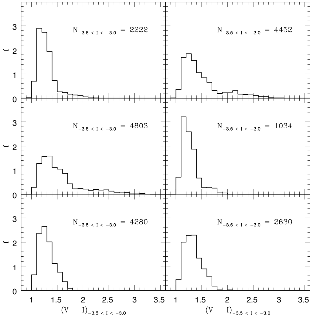
Figure G.5: Halo synthetic CMD ( V - I ) colour distribution at -3.5 < I < -3.0 for the M_{\text{tot}} = 1 \times 10^{12} M_{\odot} semi-cosmological simulations in Renda et al. (2005b). Each panel also shows the number of generated stars at -3.5 < I < -3.0 in each synthetic CMD.
