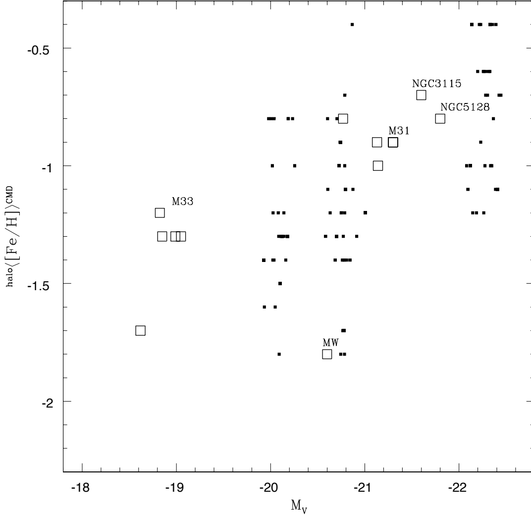
Figure 3.18: The stellar halo metallicity–total galactic V–band luminosity relation ( {}^{\text{halo}}\langle[\text{Fe}/\text{H}]\rangle^{\text{CMD}} - M_V ). A filled box corresponds to the peak of the MDF which is derived out of the (V - I) colour distribution at -3.5 < I < -3.0 via metallicity–colour relationship through the same pipeline as in Mouhcine et al. (2005). The metallicity of each artificial star of the ensemble the MDF refers to is derived via metallicity–colour relationship out of the (V - I) colour of the generated star in the RGB of the simulated “topographical” halo CMD at -3.5 < I < -3.0 . The related (V - I) colour distributions are displayed in Appendix G whereas the related MDFs derived via metallicity–colour relationship are shown in Appendix H. The observational data label–code is as in Fig. 3.1.
