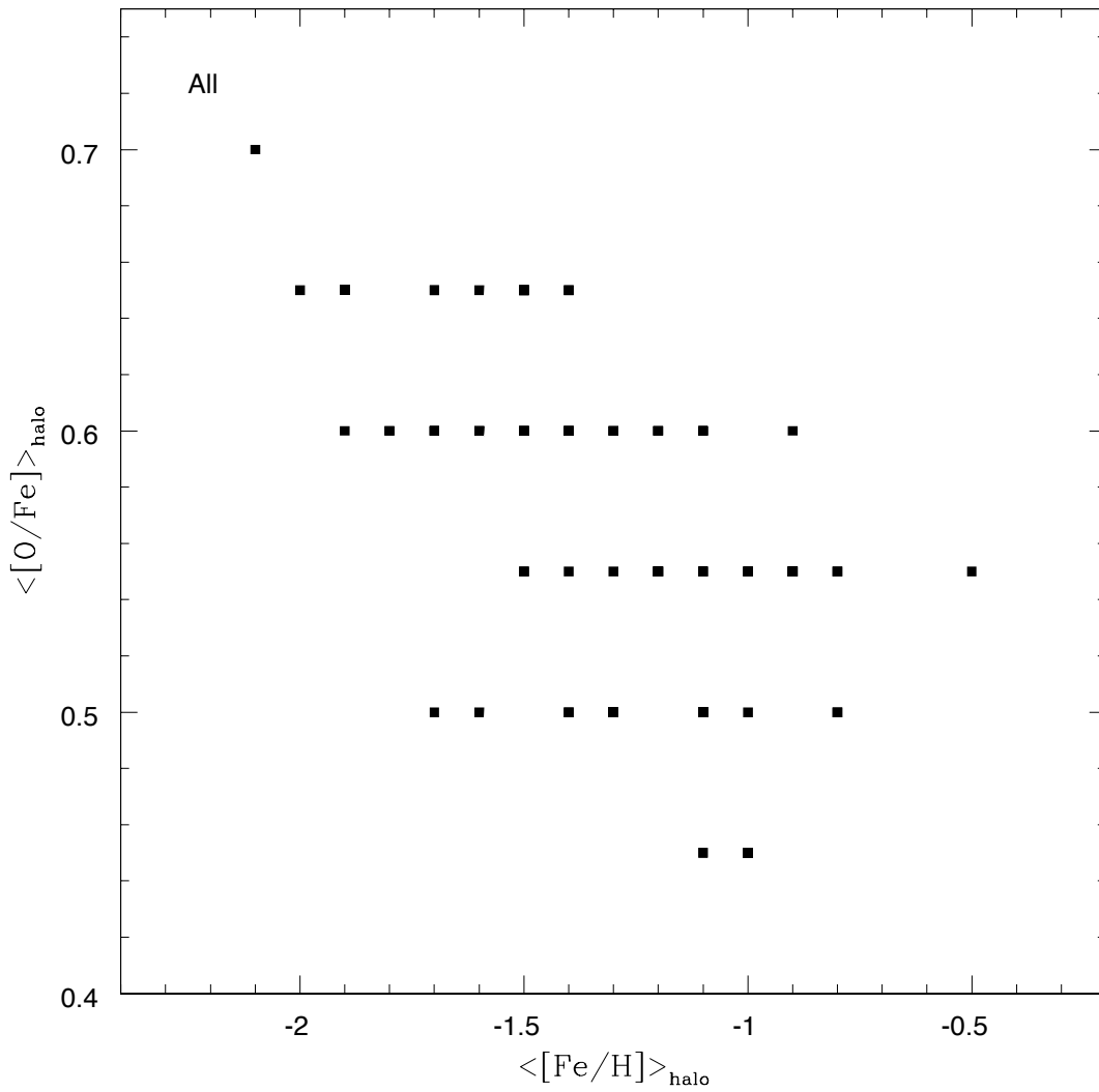
Figure 3.8: The relation between the peak of the halo [O/Fe] distribution and the peak of the halo MDF in our simulations. The related MDFs are displayed in Appendix B. The halo [O/Fe] distributions are displayed in Appendix C.
