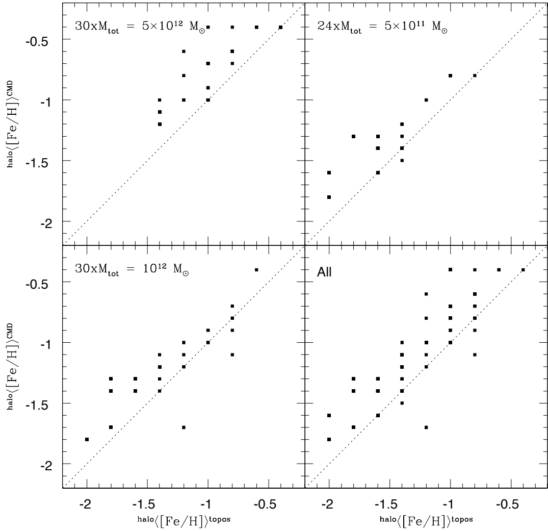
Figure 3.19: The relationship between \text{halo}\langle[\text{Fe}/\text{H}]\rangle^{\text{topos}} (the “topographical” halo metallicity) and \text{halo}\langle[\text{Fe}/\text{H}]\rangle^{\text{CMD}} (the “topographical” halo metallicity as derived from the halo simulated CMD via metallicity–colour relationship).
