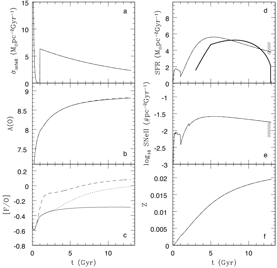
Figure A.3: Predicted evolution in the solar neighbourhood of: “a”, the gas infall rate \dot{\sigma}_{infall} ; “b”, A(O) ; “c”, [F/O] ; “d”, the star formation rate (SFR); “e”, the SNe II rate; “f”, the metallicity Z (MWa, solid line; MWb, dotted; MWc, short-dashed). The SFR history at the solar neighbourhood obtained by Bertelli & Nasi (2001) is also shown as a thick solid line in panel “d”, while the shaded region shows the range of values suggested by Rana (1991). A range of values corresponding to the estimated SNe II rate is shown in panel “e” (Cappellaro et al. 1999).
