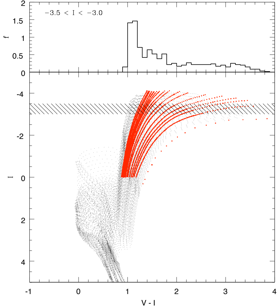
Figure 3.14: The Padova theoretical isochrones (Girardi et al., 2002) up to the RGB tip in the metallicity range of 0.0001 < Z < 0.030 which have been used to generate the simulated CMD out of the ensemble of stellar particles in the “topographical” halo for each galaxy simulation. They are shown as black dots. Red dots display the fiducial RGB tracks (i.e. 0.8 M_{\odot} VandenBerg et al. 2000 RGB tracks and the empirical NGC 6791 RGB track) which are used, as in Mouhcine et al. (2005), to construct a metallicity–colour relationship to derive [\text{Fe}/\text{H}] out of the (V - I) colour of each (generated) star in the RGB of the (simulated) CMD at -3.5 < I < -3.0 (i.e. the shaded region). The histogram in the top panel displays the (V - I) colour distribution for the Padova theoretical isochrones at -3.5 < I < -3.0 .
