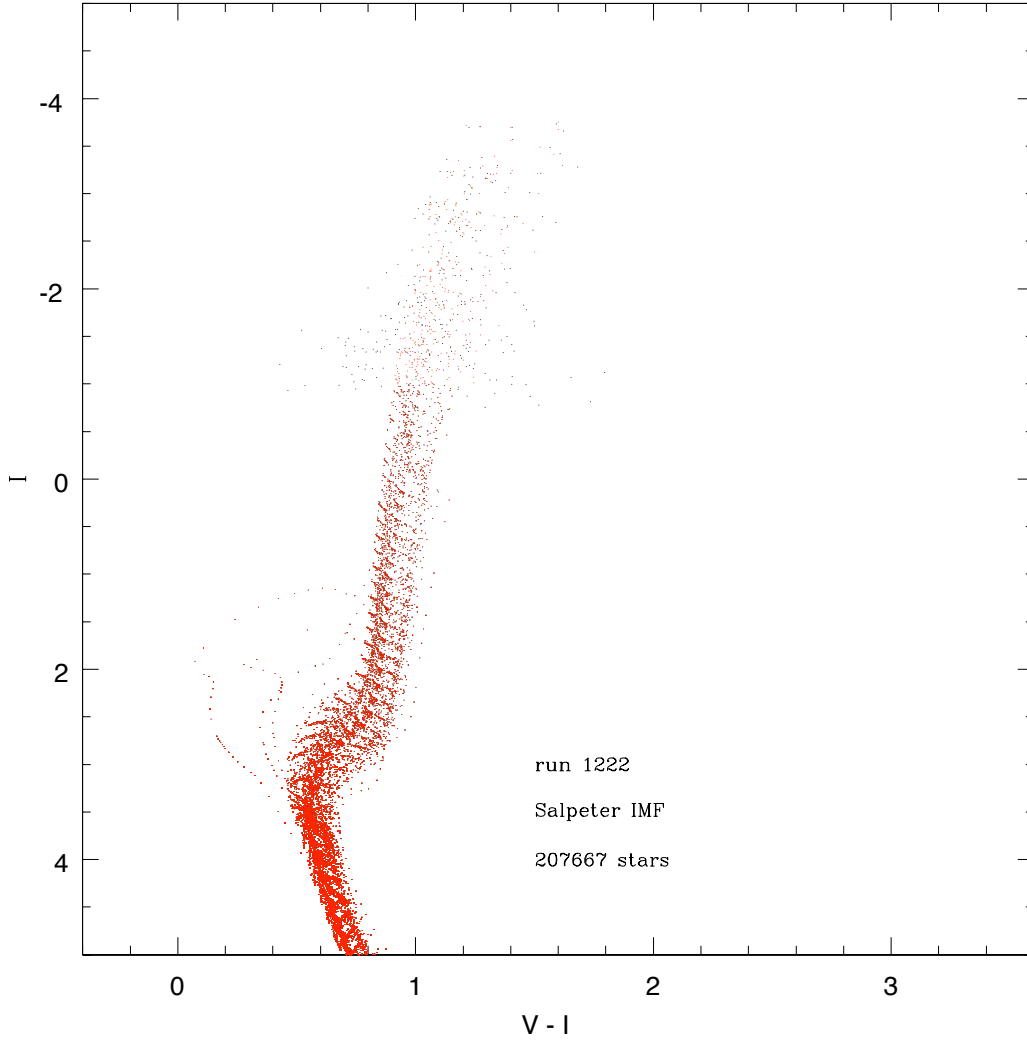
Figure 3.16: Topographical halo simulated CMD for the label “B” semi-cosmological simulation (Figures 3.5 and 3.9) at M_{\text{tot}} 10^{12} M_{\odot} . The observational errors are taken into account (e.g., Secker & Harris 1993) and are randomly drawn for I < -1 from a Normal distribution with \sigma_I = \sigma_V = \exp(I - 0.6) and \sigma_{V-I} = \sqrt{\sigma_I^2 + \sigma_V^2} which implies \sigma_I \approx 0.01 at I = -4.0 and \sigma_I \approx 0.2 at I = -1 whereas at I > -1 \sigma_I = \sigma_V = 0 . Red dots display the simulated CMD without taking observational errors into account. Black dots display the simulated CMD when taking observational errors into account.
