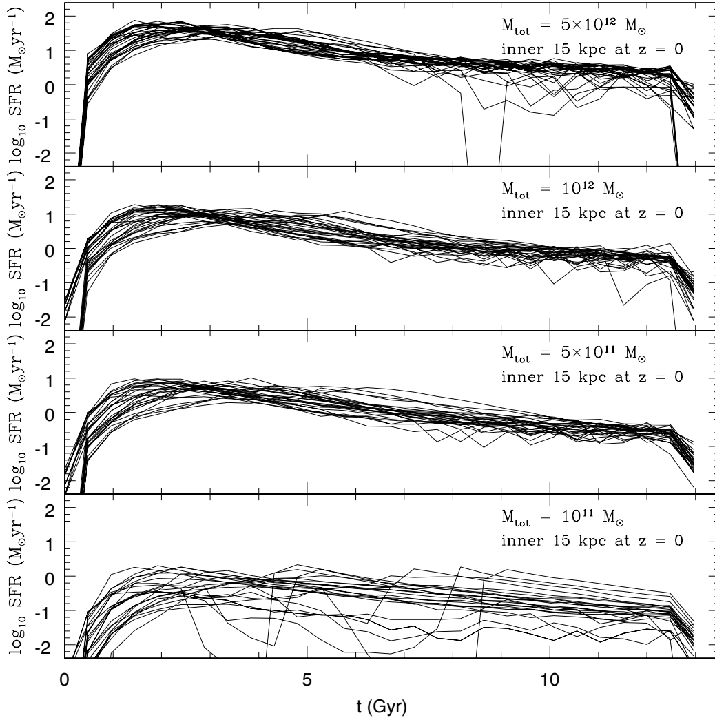
Figure 4.10: Star formation histories for each subset ( M_{\text{tot}} = : 5 \times 10^{11} M_{\odot}; 10^{12} M_{\odot}; 5 \times 10^{12} M_{\odot} ) in the simulated sample. Each star formation history refers to the ensemble of stellar particles within the inner 15 kpc at redshift z = 0 in a simulation.
