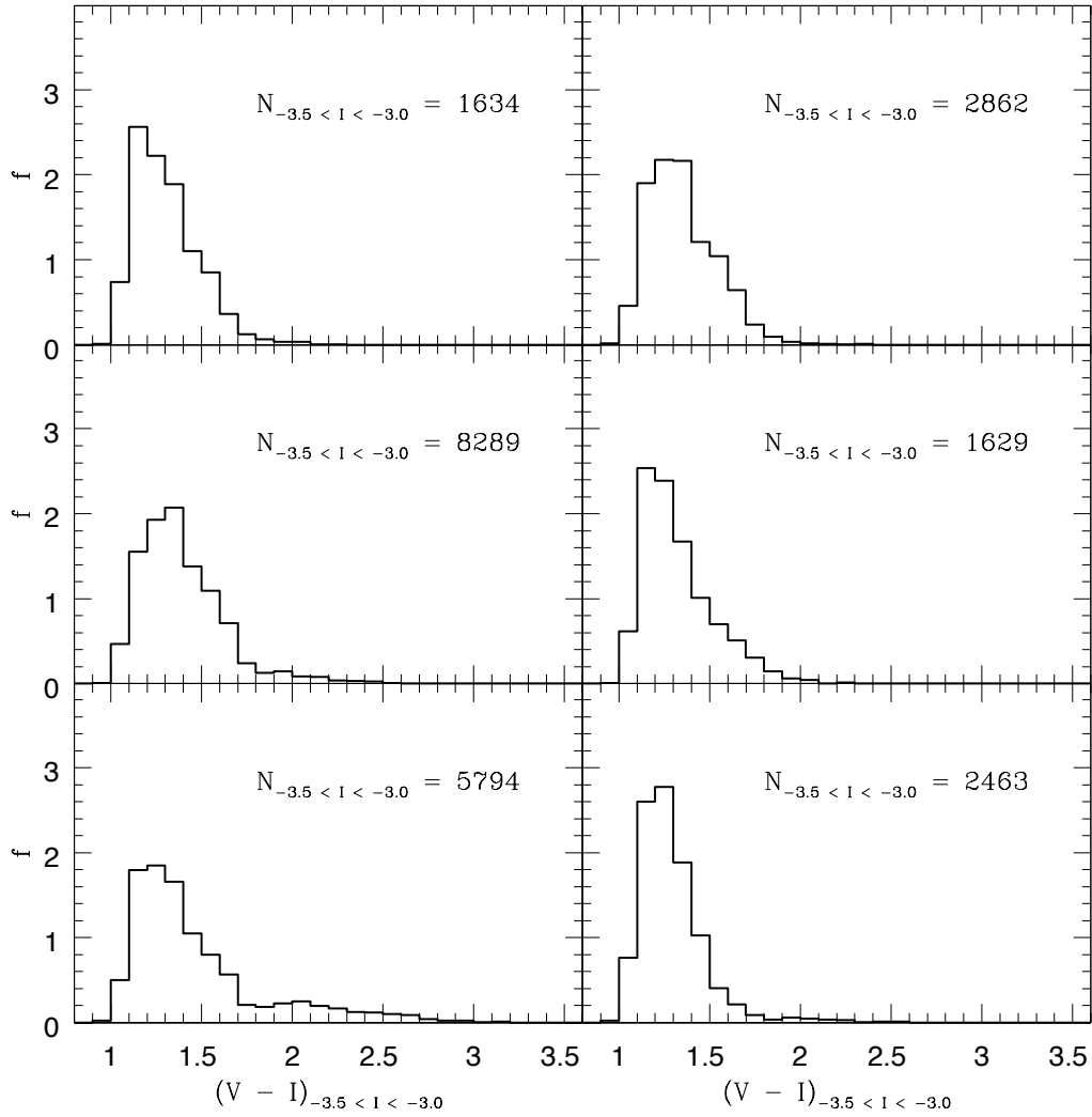
Figure G.9: (continued) Halo synthetic CMD ( V - I ) colour distribution at -3.5 < I < -3.0 for the M_{\text{tot}} = 10^{12} M_{\odot} semi-cosmological simulations in Renda et al. (2005b). Each panel also shows the number of generated stars at -3.5 < I < -3.0 in each synthetic CMD.
