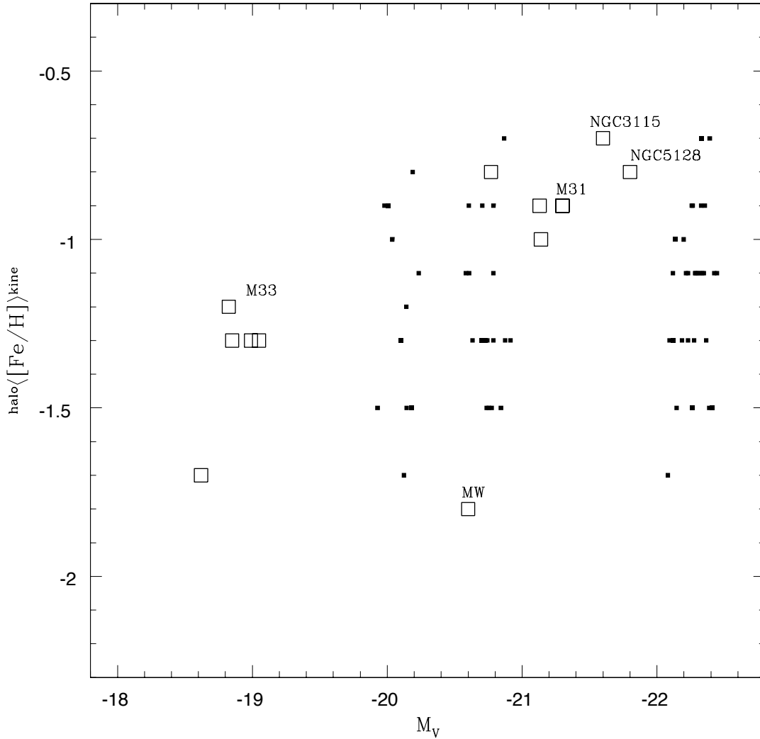
Figure 3.10: The stellar halo metallicity–total galactic V–band luminosity relation ( \langle [Fe/H] \rangle_{\text{kine}} - M_V ). A filled box corresponds to the peak of the MDF which refers, for a simulation, to the ensemble of counter–rotating ( v_\theta < 0 ) stellar particles within each topographical halo (at a projected radius R > 15 kpc). The related MDFs are displayed in Appendix F. The observational data label–code is as in Fig. 3.1.
