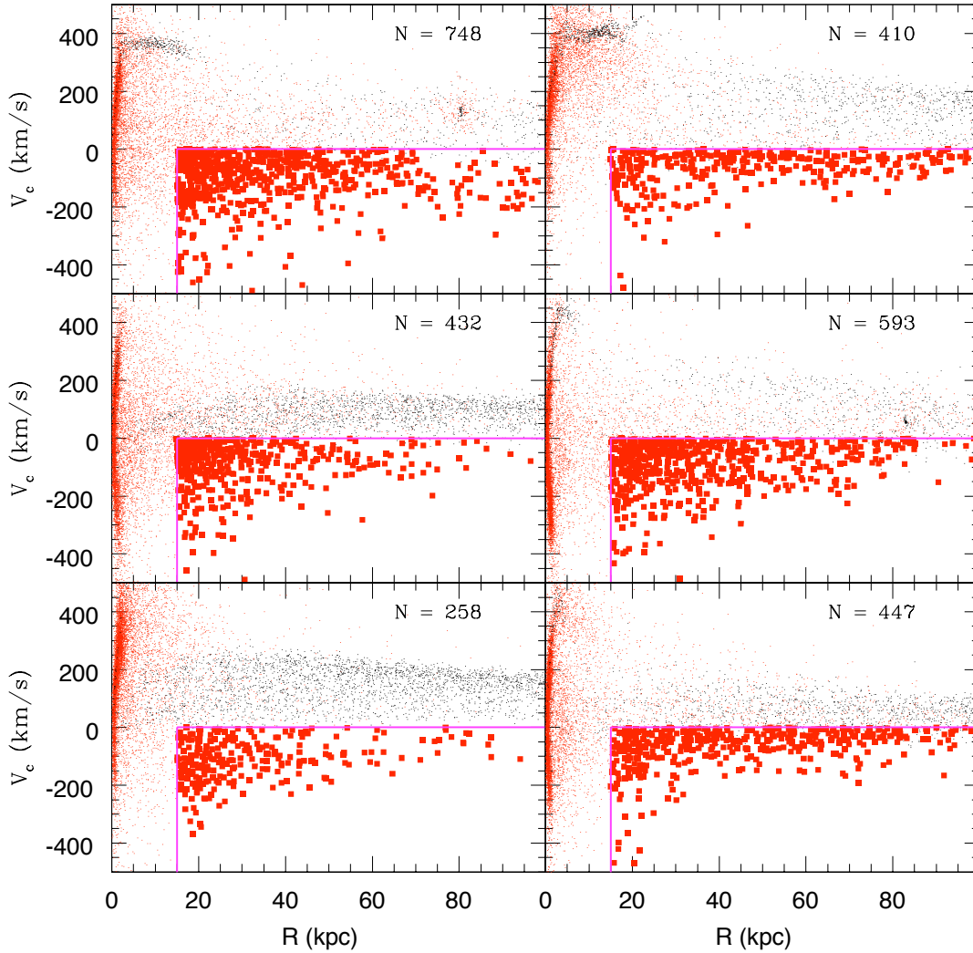
Figure E.11: (continued) Galaxy rotation curves for the M_{\text{tot}} = 5 \times 10^{12} M_{\odot} semi-cosmological simulations in Renda et al. (2005b). Black dots for the gaseous particles. Red dots for the stellar particles; red boxes for the ensemble of stellar particles (enclosed within the magenta frame) which are counter-rotating with v_{\theta} < 0 within each topographical halo at a projected radius R > 15 kpc. The size of such ensemble is also shown in each panel.
