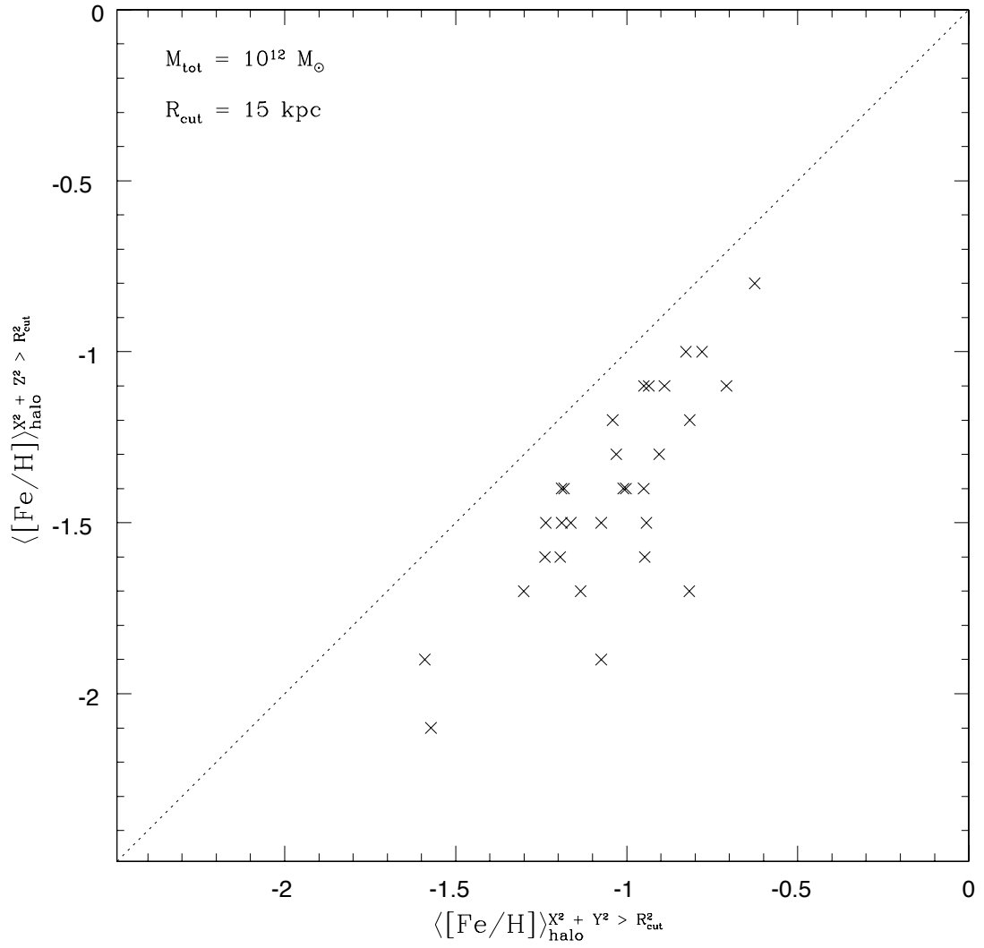
Figure 3.3: Topographical halo metallicity ( R_{\text{cut}} = 15 kpc) for the M_{\text{tot}} = 10^{12} M_{\odot} subset as a function of different halo definitions, according to either x^2 + y^2 > R_{\text{cut}}^2 or x^2 + z^2 > R_{\text{cut}}^2 .
