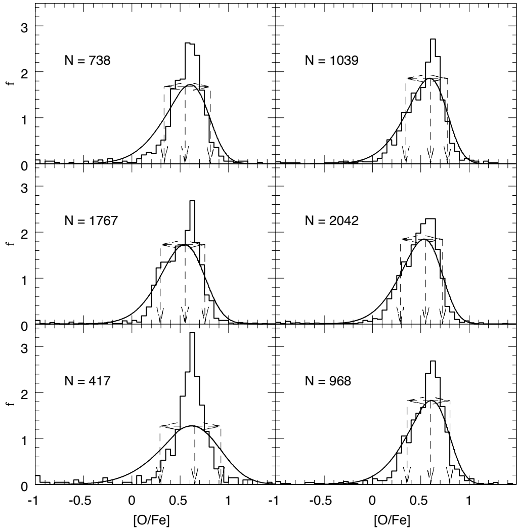
Figure C.14: (continued) Halo stellar particle [O/Fe] distribution for the M_{\text{tot}} = 5 \times 10^{12} M_{\odot} semi-cosmological simulations in Renda et al. (2005b). The 68% Confidence Level range and the number of stellar particles each distribution refers to are also shown.
