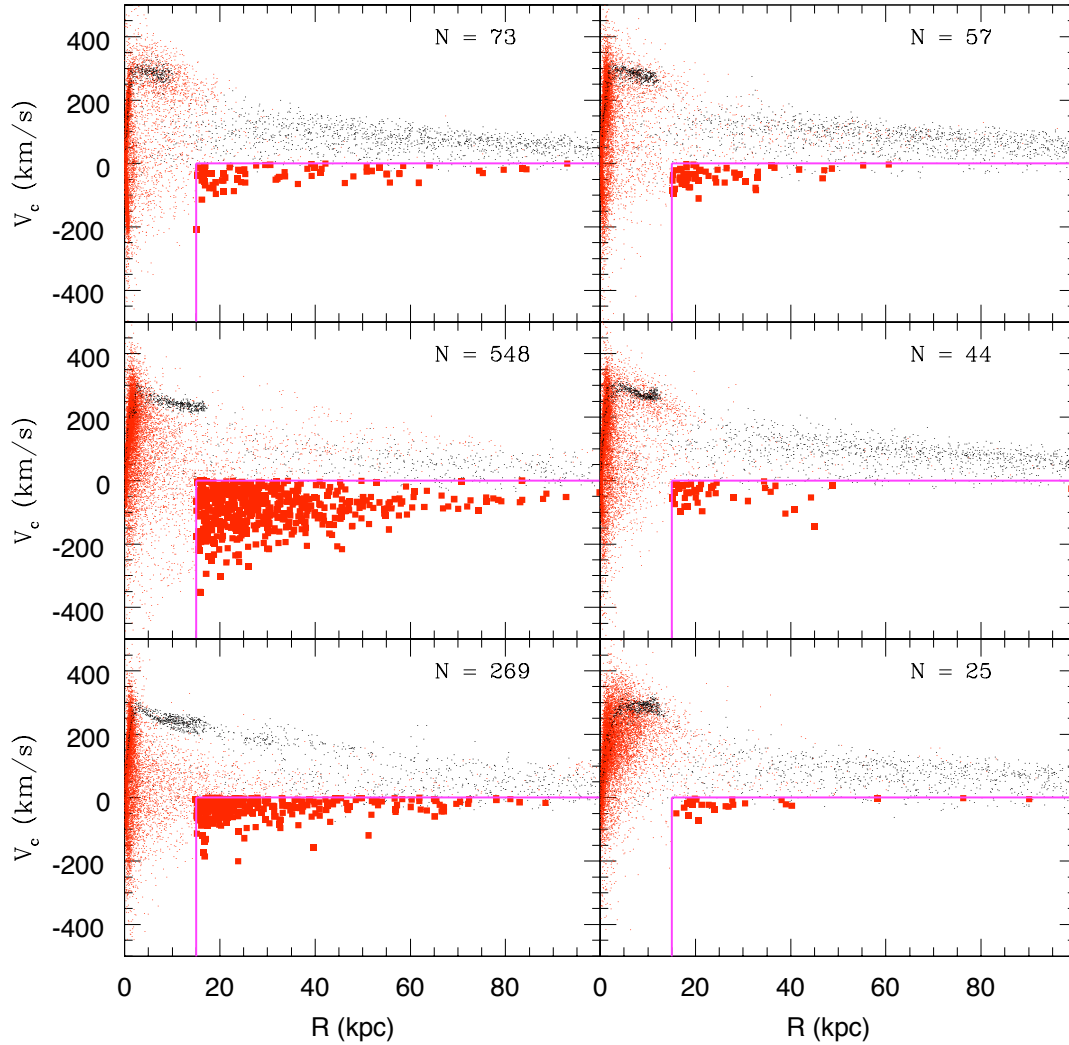
Figure E.9: (continued) Galaxy rotation curves for the M_{\text{tot}} = 10^{12} M_\odot semi-cosmological simulations in Renda et al. (2005b). Black dots for the gaseous particles. Red dots for the stellar particles; red boxes for the ensemble of stellar particles (enclosed within the magenta frame) which are counter-rotating with v_\theta < 0 within each topographical halo at a projected radius R > 15 kpc. The size of such ensemble is also shown in each panel.
