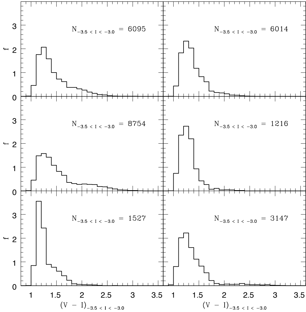
Figure G.7: (continued) Halo synthetic CMD ( V - I ) colour distribution at -3.5 < I < -3.0 for the M_{\text{tot}} = 10^{12} M_{\odot} semi-cosmological simulations in Renda et al. (2005b). Each panel also shows the number of generated stars at -3.5 < I < -3.0 in each synthetic CMD.
