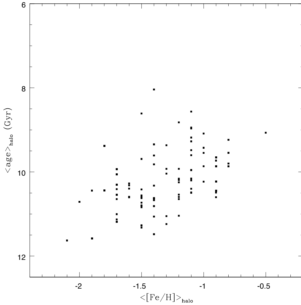
Figure 3.6: The relation between the mean stellar halo age and the peak of the halo MDF in our simulations. The halo ADFs are displayed in Appendix D.
