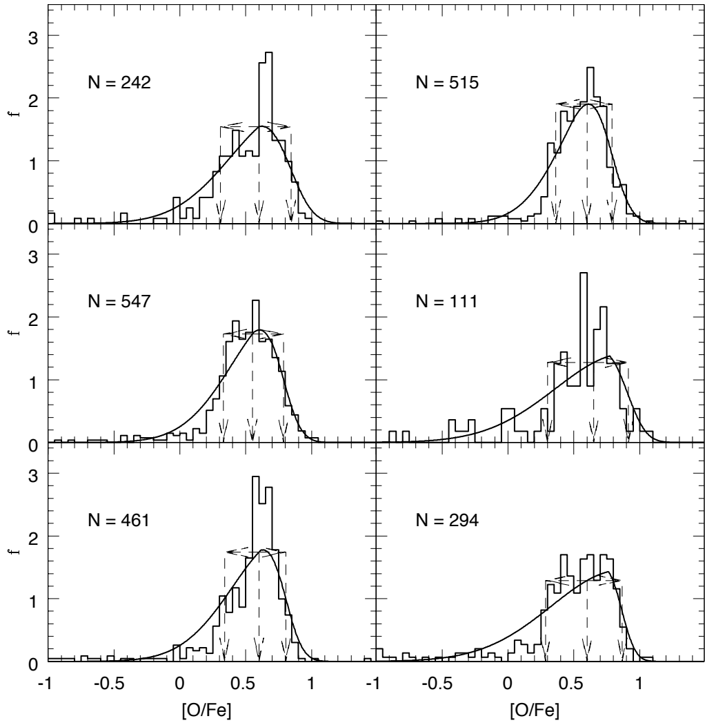
Figure C.6: Halo stellar particle [O/Fe] distribution for the M_{\text{tot}} = 1 \times 10^{12} M_{\odot} semi-cosmological simulations in Renda et al. (2005b). The 68% Confidence Level range and the number of stellar particles each distribution refers to are also shown.
