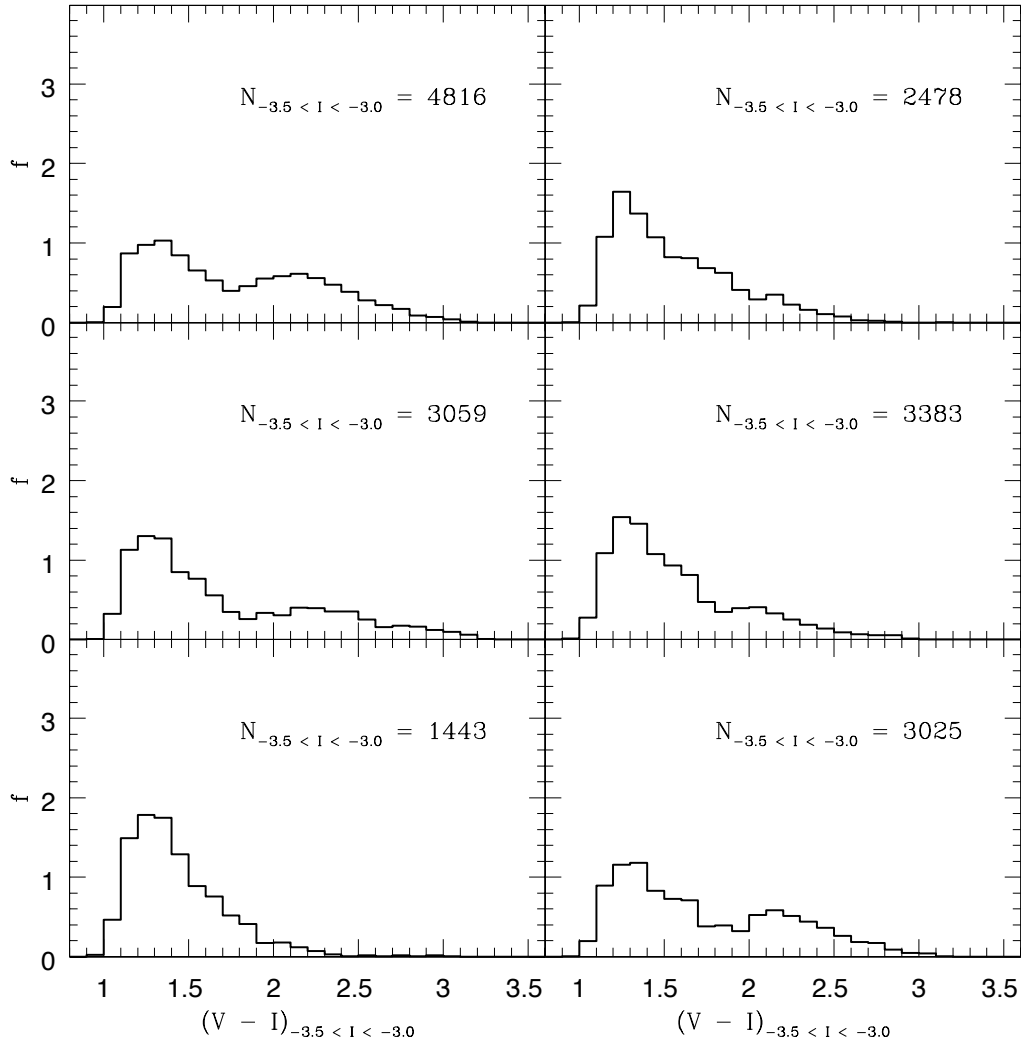
Figure G.11: (continued) Halo synthetic CMD ( V - I ) colour distribution at -3.5 < I < -3.0 for the M_{\text{tot}} = 5 \times 10^{12} M_{\odot} semi-cosmological simulations in Renda et al. (2005b). Each panel also shows the number of generated stars at -3.5 < I < -3.0 in each synthetic CMD.
