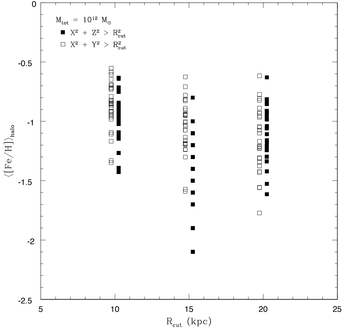
Figure 3.2: Topographical halo metallicity for the M_{\text{tot}} = 10^{12} M_{\odot} subset as a function of different halo definitions (according to either x^2 + y^2 > R_{\text{cut}}^2 , empty symbols, or x^2 + z^2 > R_{\text{cut}}^2 , filled symbols) and cut-off radii ( R_{\text{cut}} = 10 kpc; 15 kpc; 20 kpc).
