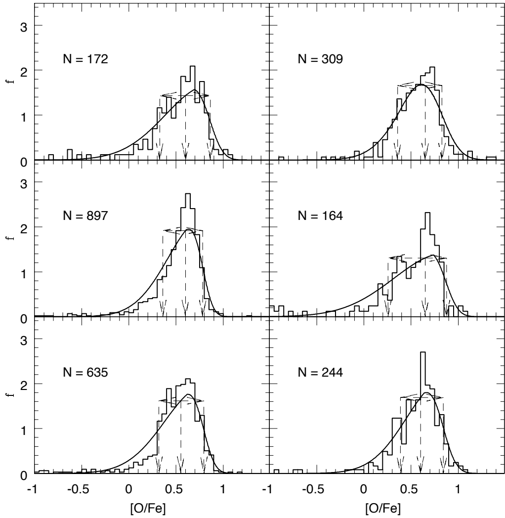
Figure C.10: (continued) Halo stellar particle [O/Fe] distribution for the M_{\text{tot}} = 10^{12} M_{\odot} semi-cosmological simulations in Renda et al. (2005b). The 68% Confidence Level range and the number of stellar particles each distribution refers to are also shown.
