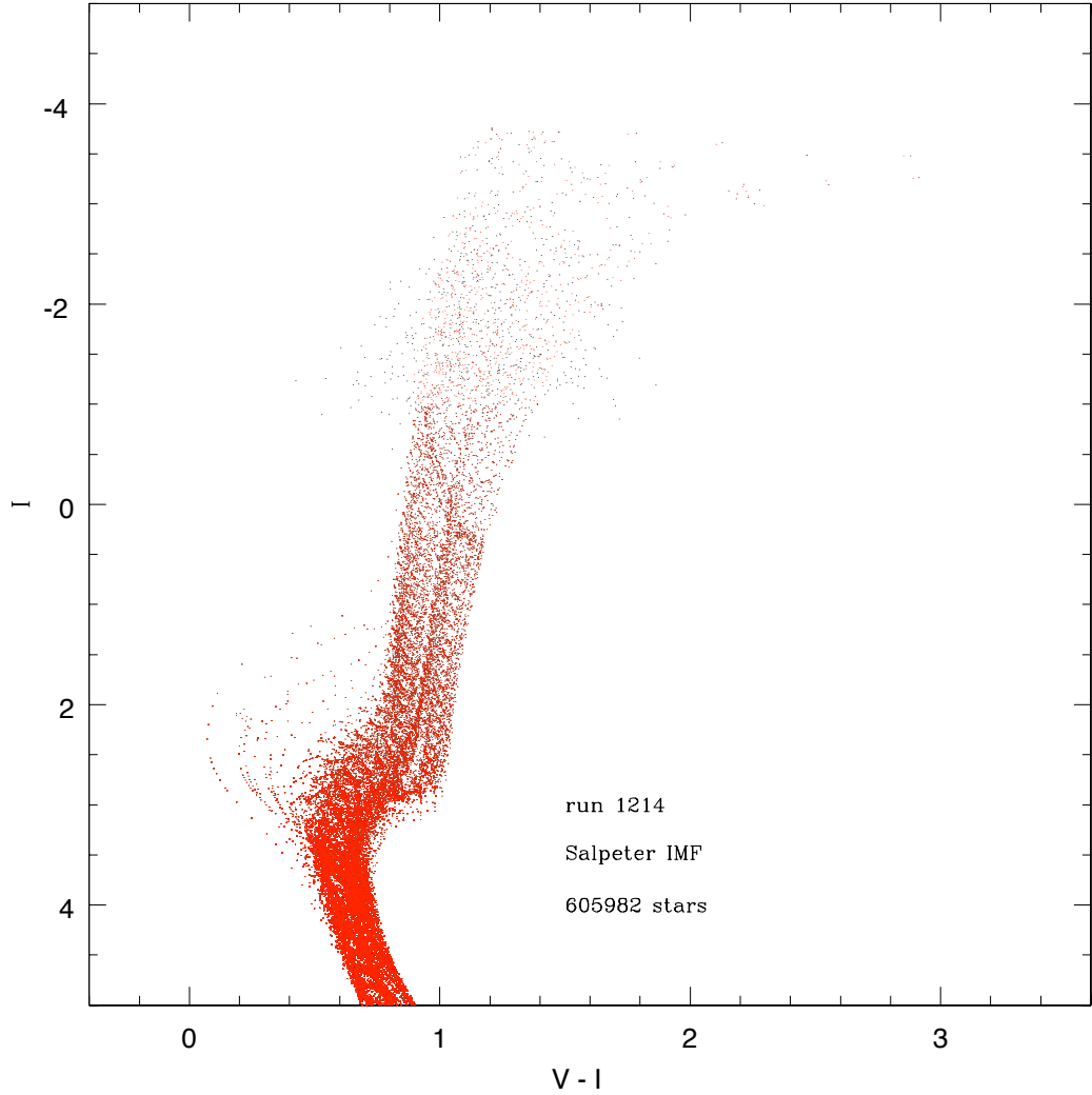
Figure 3.15: Topographical halo simulated CMD for the label “A” semi-cosmological simulation (Figures 3.5 and 3.9) at M_{\text{tot}} 10^{12} M_{\odot} . The observational errors are taken into account (e.g., Secker & Harris 1993) and are randomly drawn for I < -1 from a Normal distribution with \sigma_I = \sigma_V = \exp(I - 0.6) and \sigma_{V-I} = \sqrt{\sigma_I^2 + \sigma_V^2} which implies \sigma_I \approx 0.01 at I = -4.0 and \sigma_I \approx 0.2 at I = -1 whereas at I > -1 \sigma_I = \sigma_V = 0 . Red dots display the simulated CMD without taking observational errors into account. Black dots display the simulated CMD when taking observational errors into account.
